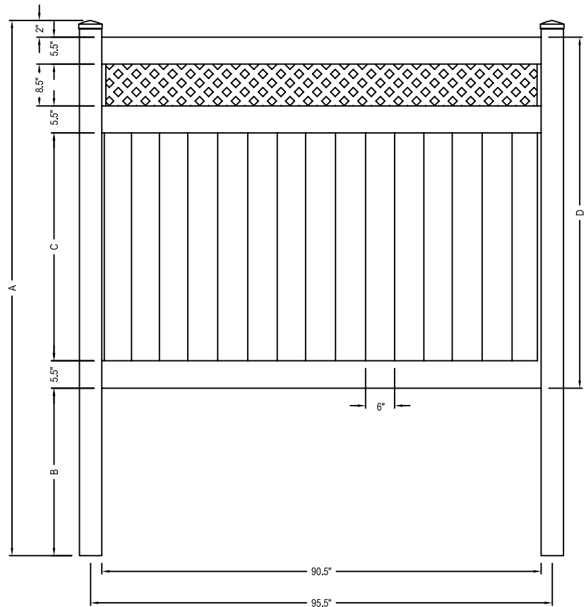
FRONT ELEVATION
