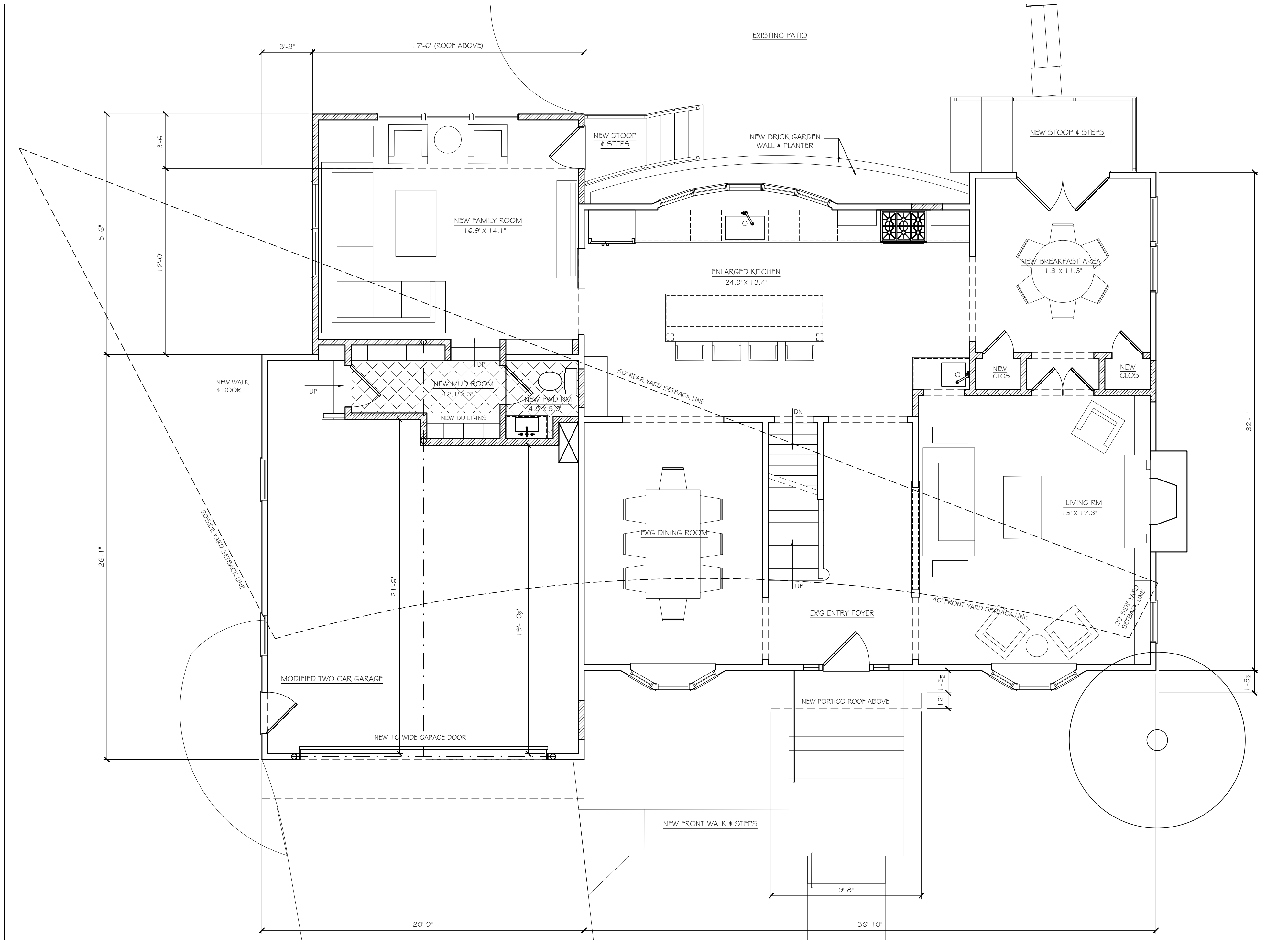
1 PROPOSED FIRST FLOOR PLAN A3 SCALE: 1/4" = 1'-0"
