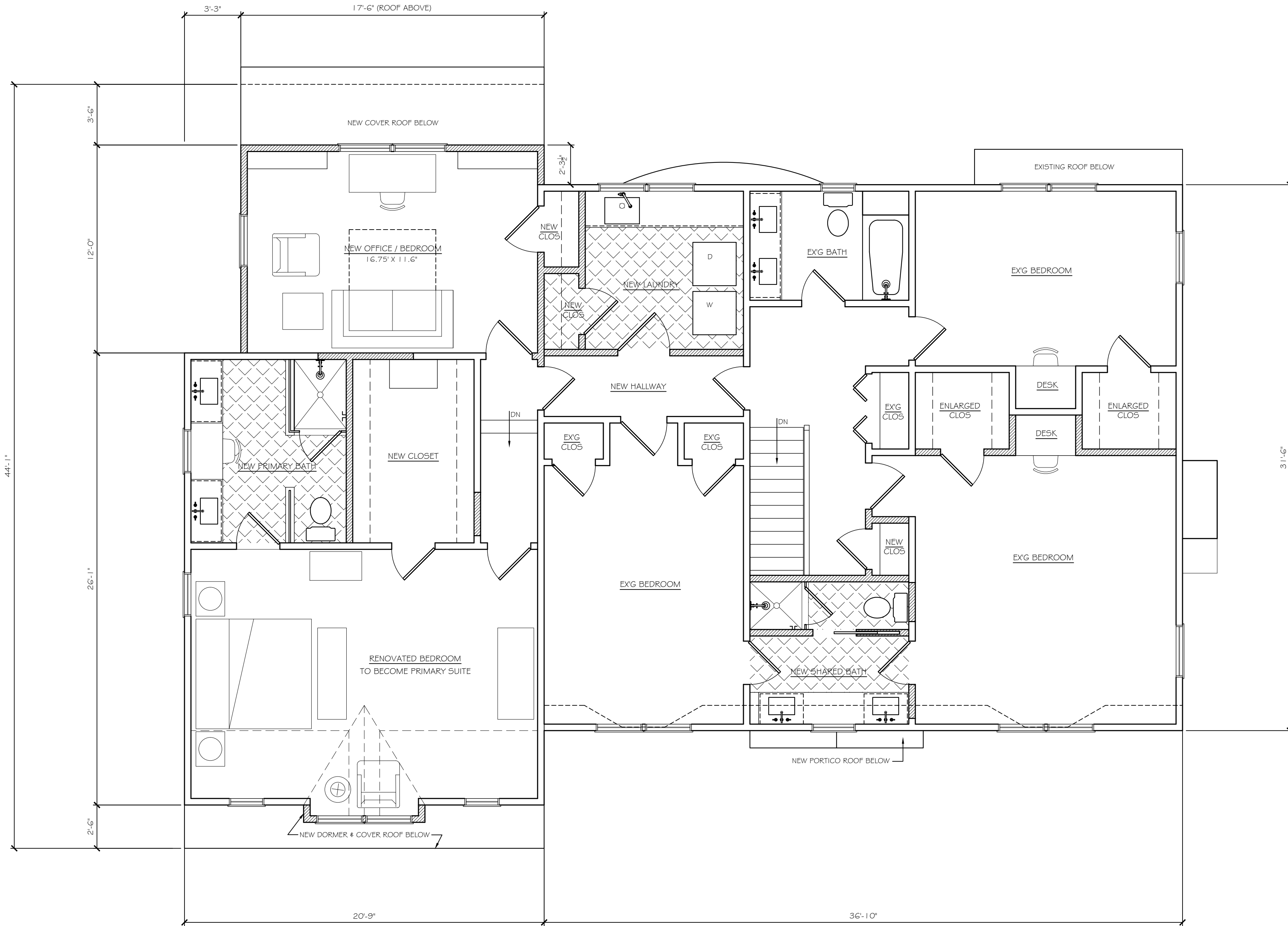
1 A4 PROPOSED SECOND FLOOR PLAN SCALE: 1/4" = 1'-0"
